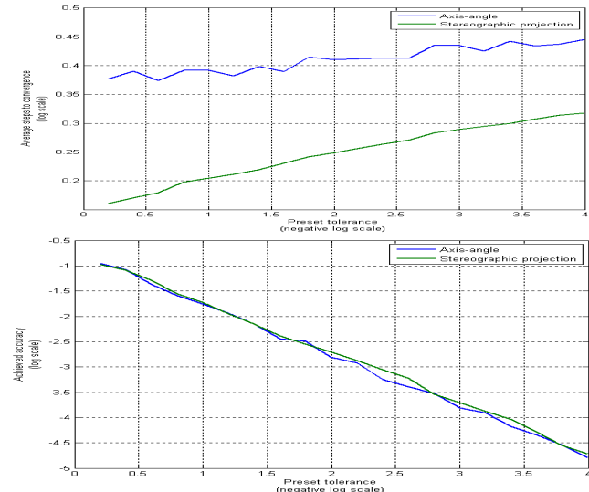
Fig. 3. Performance comparison in the context of LM iteration with a fixed starting point for 20 error tolerance values (negative log scale). a) Plot of average number of steps (log scale) required to reach the preset tolerance. b) Plot of average error norm(log scale) following convergence.
