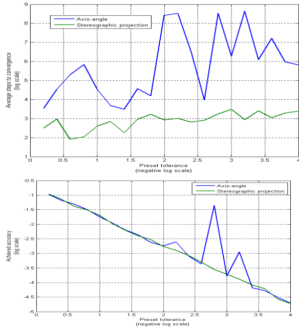
Fig. 4. Performance comparison in the context of LM iteration with random starting point for 20 error tolerance values (negative log scale). a) Plot of average number of steps (log scale) required to reach the preset tolerance. b) Plot of average error norm (log scale) following convergence.
