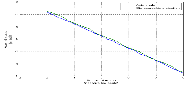
Fig. 5. Performance comparison in the context of LM iteration for randomly generated quaternions in the neighborhood of the south pole. a) Plot of average number of steps required to reach the preset tolerance. b) Plot of average error norm (log scale) following convergence.
