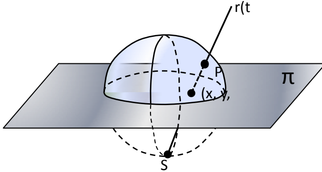
Fig. 1. The 4D spherical hypersurface of unit quaternions visualized as a 3D sphere. Point S is the center of projection and (x, y, z) a point on the 3D hyperplane. The ray r(t) intersects the surface of the sphere at P .
