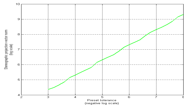
Fig. 6. Average norm of the stereographic projection parameter vector for preset tolerance in the range of 10^{-3} to 10^{-8} .
