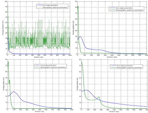
Fig. 2. The average gradient norm plots for a sequence of 10 steepest descent executions regarding the estimation of a randomly generated rotation matrix. a) Learning rate a=0.01 , b) Learning rate a=0.001 , c) Learning rate a=0.0006 , d) Learning rate a=0.0003 .
